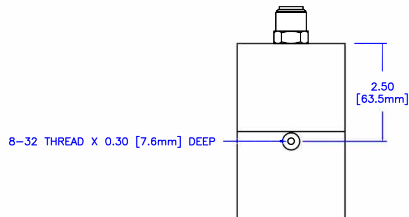
BOTTOM VIEW
