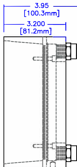
SIDE VIEW
