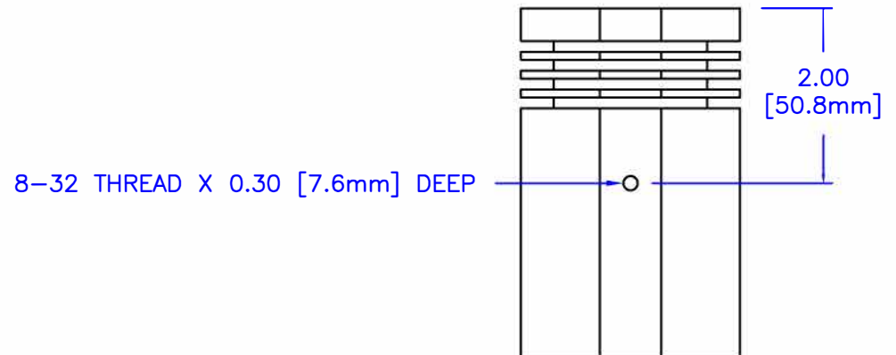
BOTTOM VIEW
